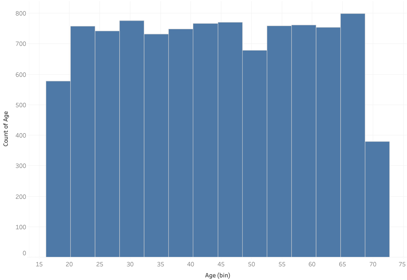
The trend of count of Age for Age (bin).
